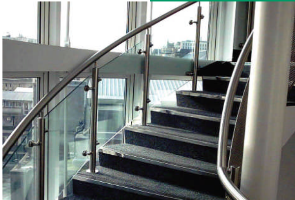
Curved balustrade with glass and perforated sheet infill panel
